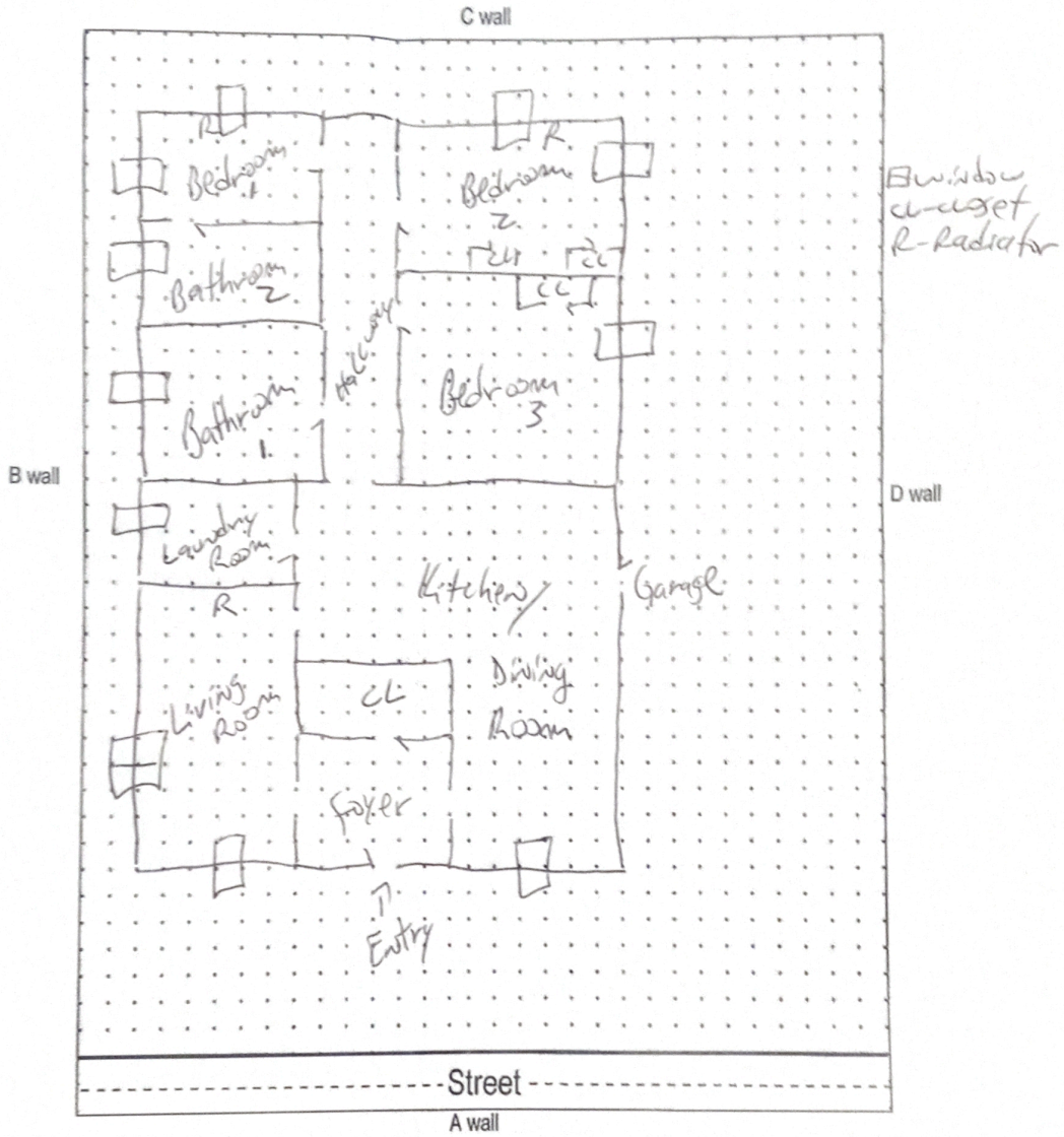
Floor 1
